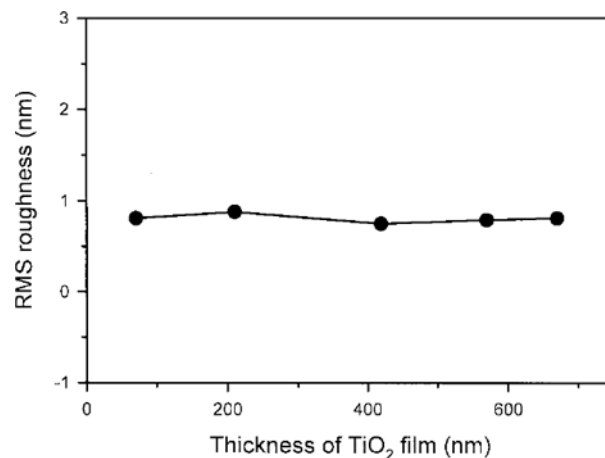
Fig. 5. RMS roughness of sol-gel derived TiO 2 films in various thicknesses.
