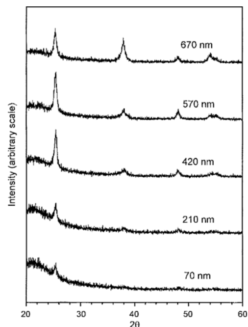
Fig. 2. XRD patterns of TiO 2 films in various thicknesses. Sol-gel derived TiO 2 films were annealed at 500 °C for 1 hr.
